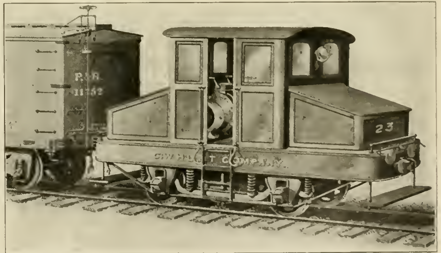
ELECTRIC LOCOMOTIVE FOR STANDARD GAUGE.
